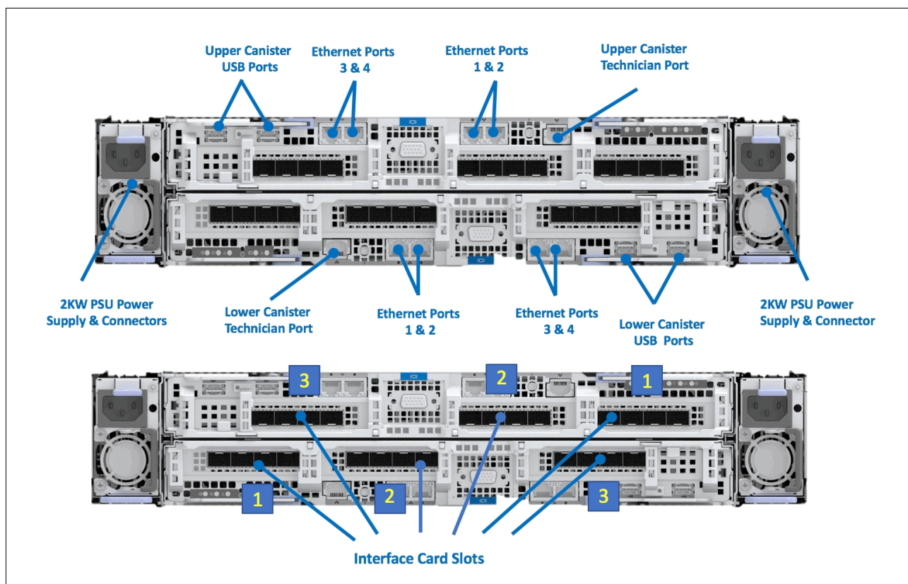
Figure 13 Rear view of IBM FlashSystem 7300 control enclosure
