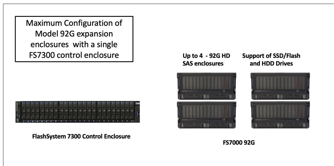
Figure 20 Maximum configuration for model 92G enclosures
